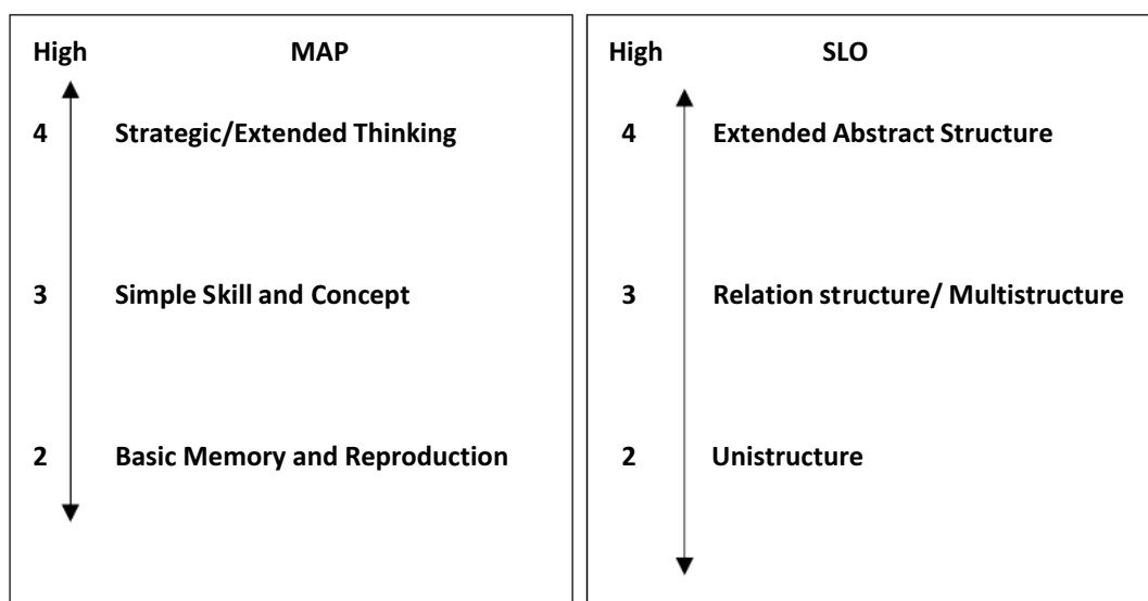
Figure 1. Construct maps
